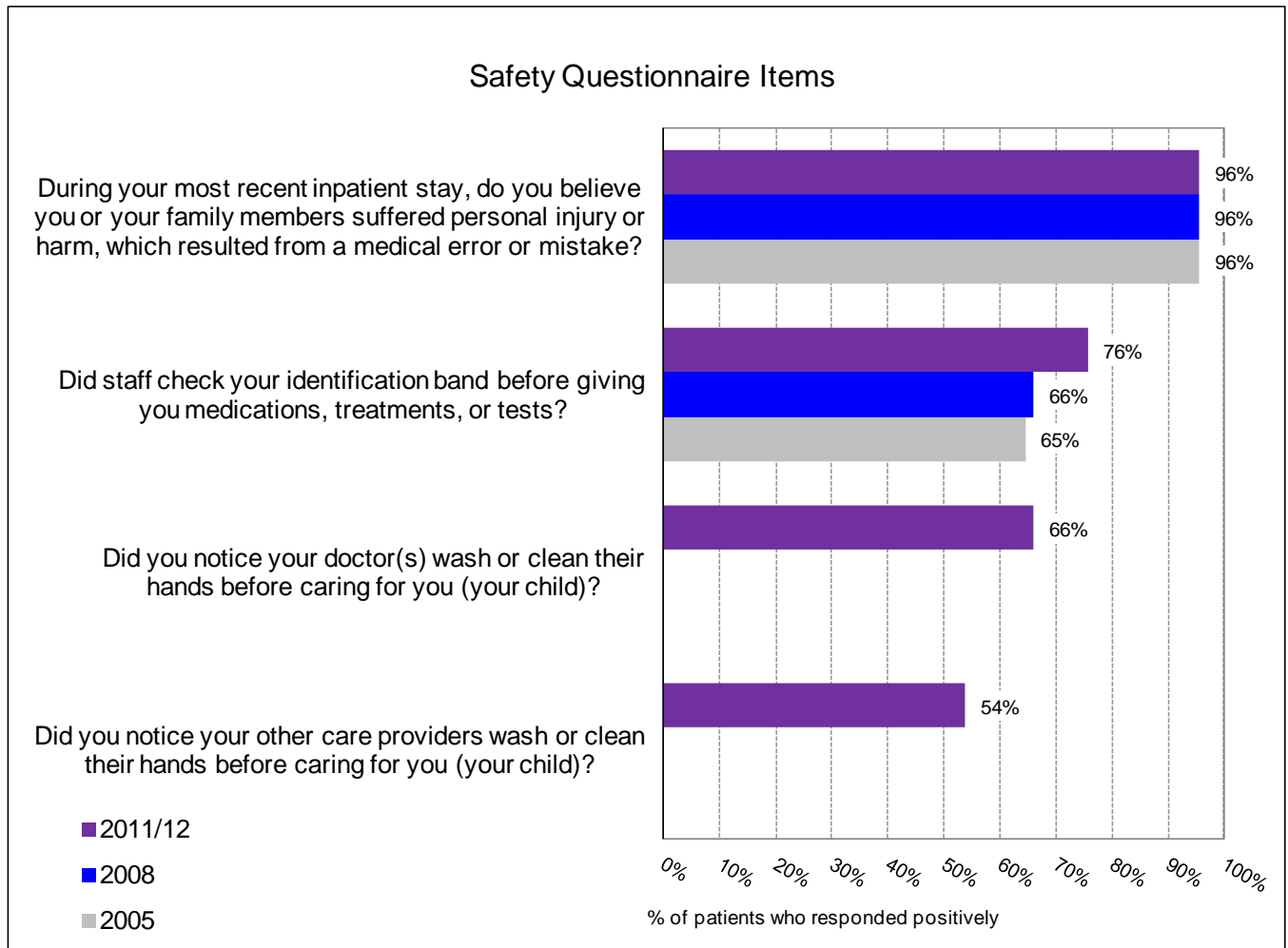
Figure 25: Safety Questions
